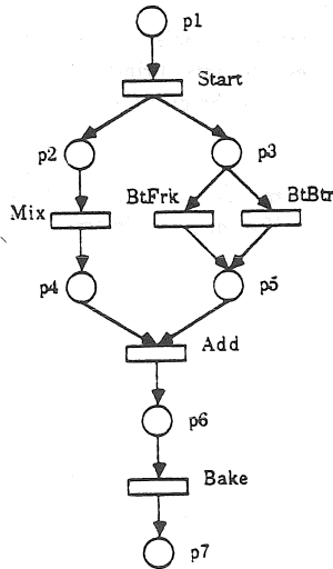
Figure 1: Graphical representation of ER-net V .
