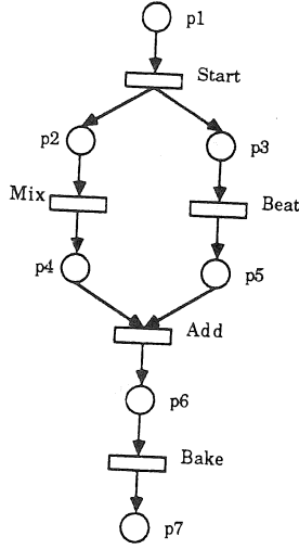
Figure 9: The recipe after parallel decomposition.
