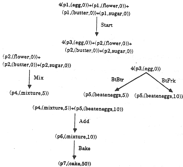
Figure 2: Graphical representation of the ER-graph \mathcal{G}[N] .
