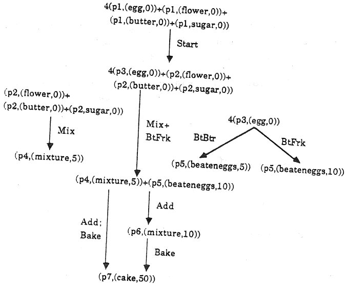
Figure 3: Graphical representation of the ER-computation graph C[N] .
